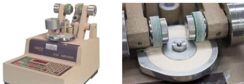
Figura 06: Taber abrasion.
