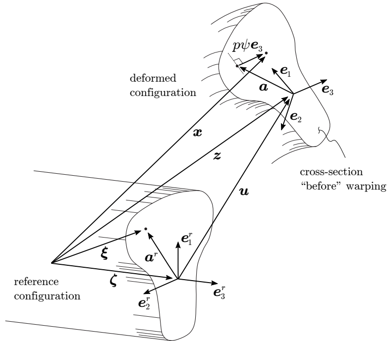
Figure 1: Rod description and kinematics. Source: created by the authors.
